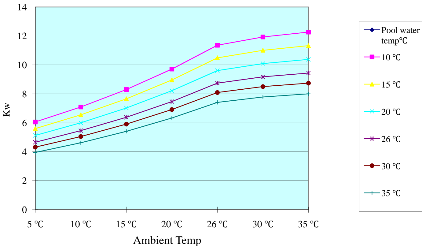
THP09 heating capacity at different air & water temperature
